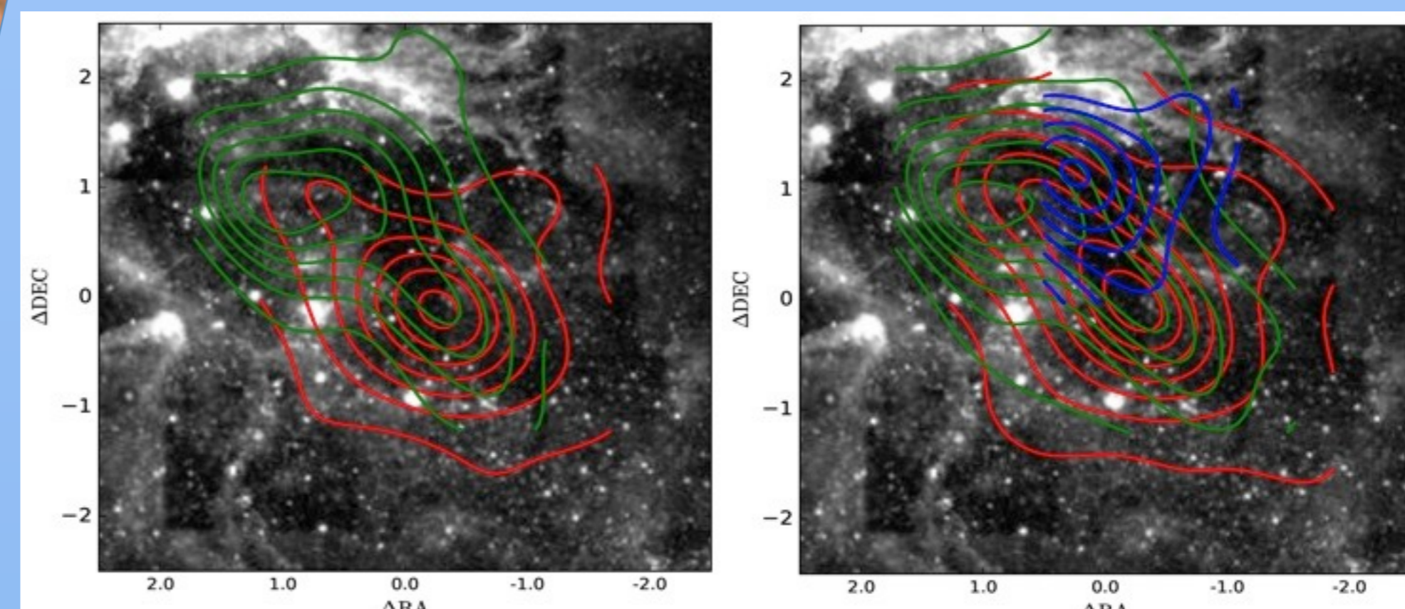
Fig. 3: WISE gray image showing the iso-density contours for each group using a cutoff of 1.4 (LEFT) and 1.5 (RIGHT) with the OPTICS algorithm. You can see the corresponding central values of RV for each group in the table 1.
