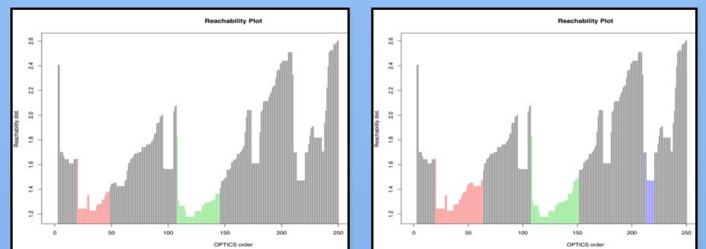
Fig. 4: The reachability plot obtained with OPTICS algorithm, using a cutoff of 1.4 (LEFT) and 1.5 (RIGHT) to show the substructures of the phase space. We found two and three groups, respectively. You can find the mean values of RV for each group in table 1.
