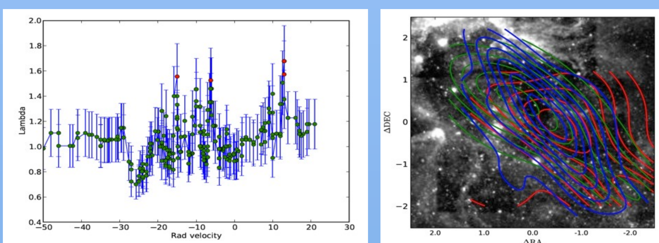
Fig. 2: (LEFT) The kinematic index Lambda versus the central RV showing with red dots the spatially segregated groups. (RIGHT) WISE gray image showing the iso-density contours for each group with RV median of -15.0 km/s (green), -6.2 km/s (red), and 13.0 km/s (blue), respectively.
