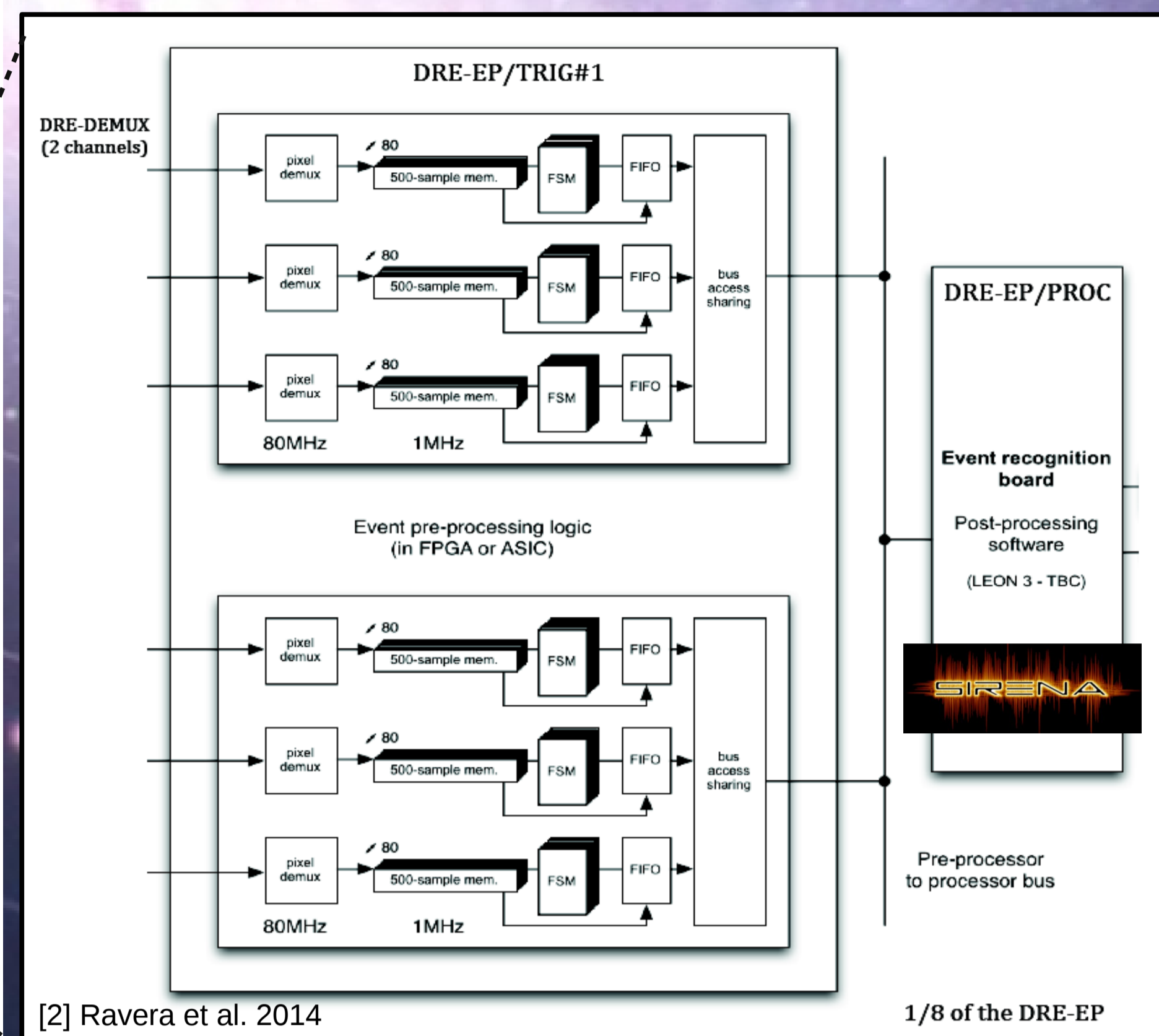
Pulses must be detected (triggered) and then its energy must be reconstructed on board by the Event Processor in the Digital Readout Electronics Unit by the SIRENA software
