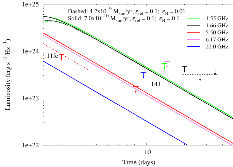
Figure 1: Predicted radio light curves of SN 2014J in M 82 for an assumed mass-loss rate of \dot{M} = 7.0 \times 10^{-10} M_{\odot} \text{ yr}^{-1} (solid lines), and for \dot{M} = 4.2 \times 10^{-9} M_{\odot} \text{ yr}^{-1} (dashed lines). For the former we used \epsilon_B = 0.1 and for the latter \epsilon_B = 0.01 . The data points (cf. Table 1) with 3\sigma upper limits for SN 2014J are in the right part of the figure. Shown in the figure is also the earliest 5.9 GHz 3\sigma upper limit for SN 2011fe [4], scaled to its distance of 6.4 Mpc, together with a dotted line marking the predicted evolution for \dot{M} = 5.0 \times 10^{-10} M_{\odot} \text{ yr}^{-1} (for \epsilon_B = 0.1 ). Common parameters in all models are \epsilon_{\text{rel}} = 0.1 , p = 3 and v_w = 100 \text{ km s}^{-1} . See text for further details.
